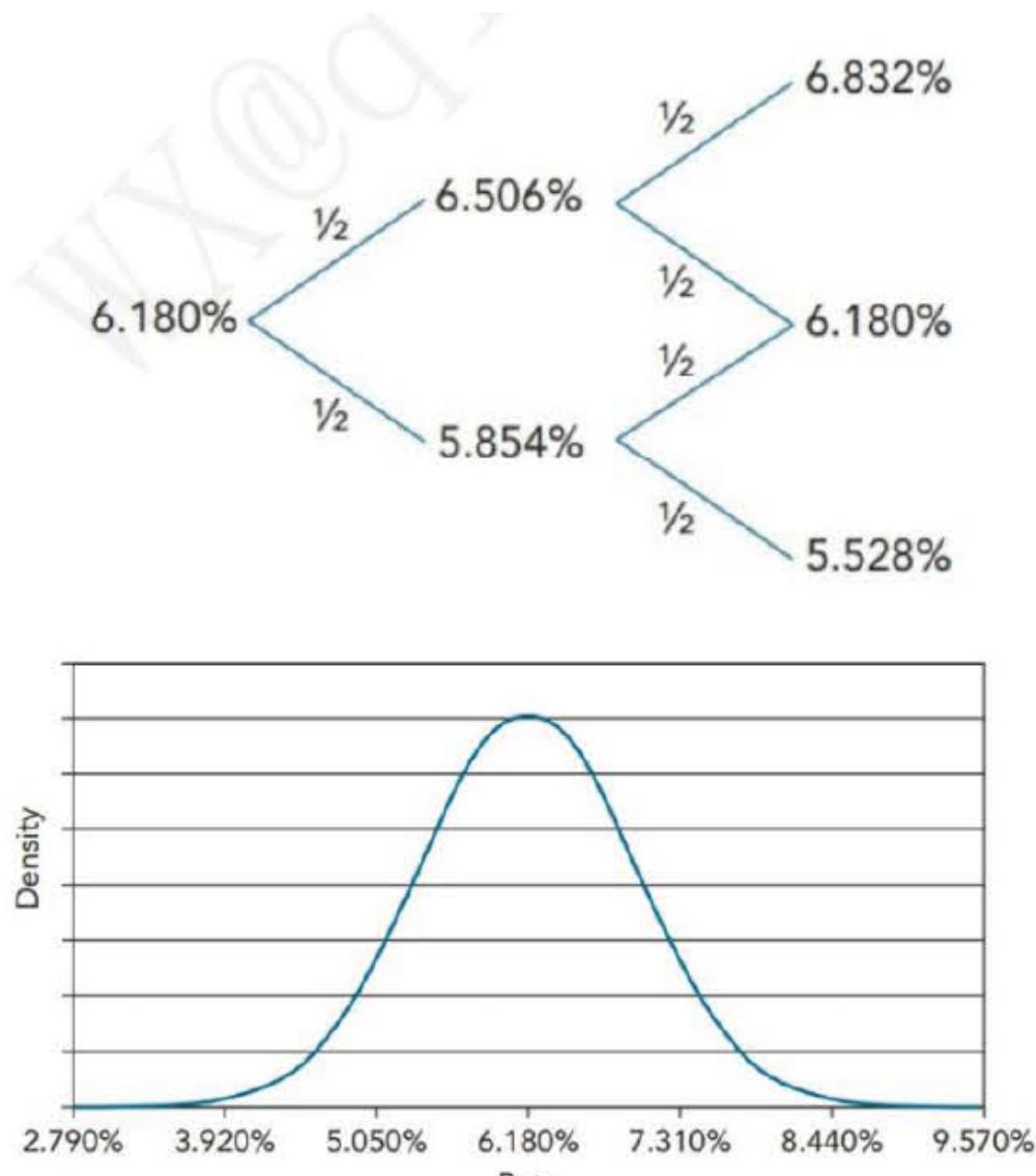
(Distribution of short rates after one year, Model 1)
